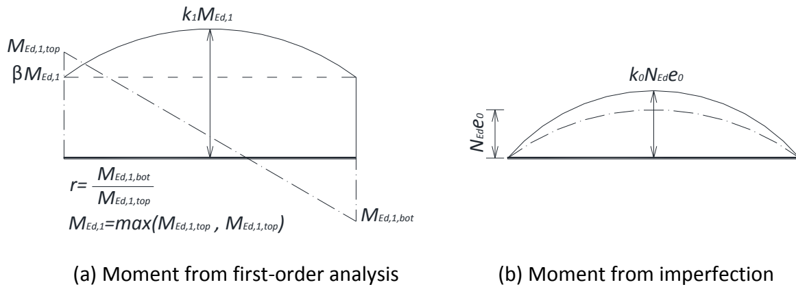
Figure 6: Consideration for second order effect
