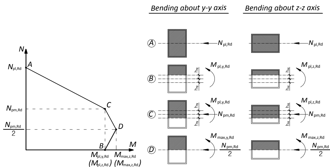
Figure 10: Simplified interaction curve for rectangular CFST columns
