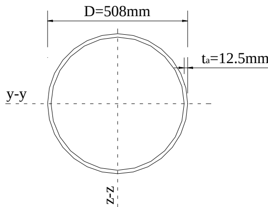
Figure 1: Cross-sectional dimensions of CFST column in Example 1
